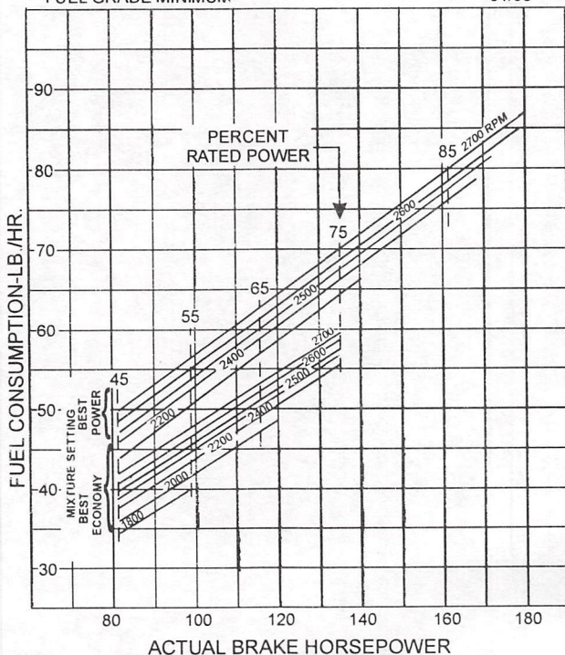
Figure 3-7. Part Throttle Fuel Consumption – IO-360-B, -E, -F, -M1A Series (Excepting IO-360-B1A, -B1C)
