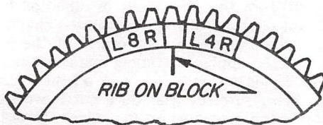
Figure 5-2. Timing Marks - 4 cyl. 1200 Series
