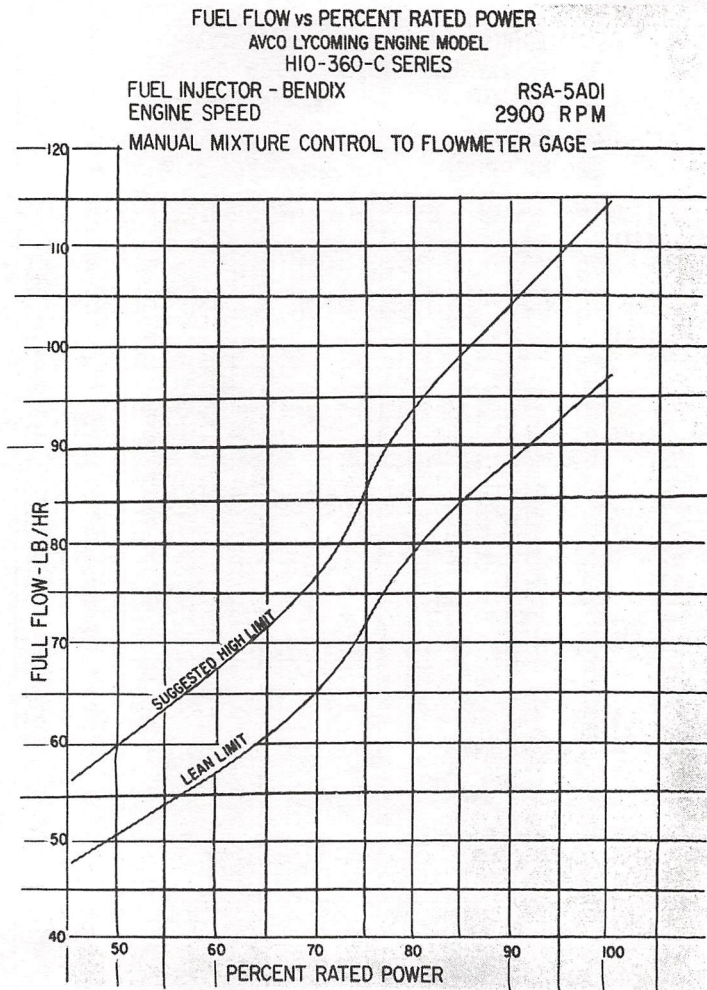
Figure 3-16. Fuel Flow vs Percent Rated Power H10-360-C Series
