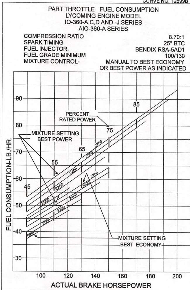
Figure 3-6. Part Throttle Fuel Consumption - IO-360-A, -C, -D, -J, -K; AIO-360 Series
