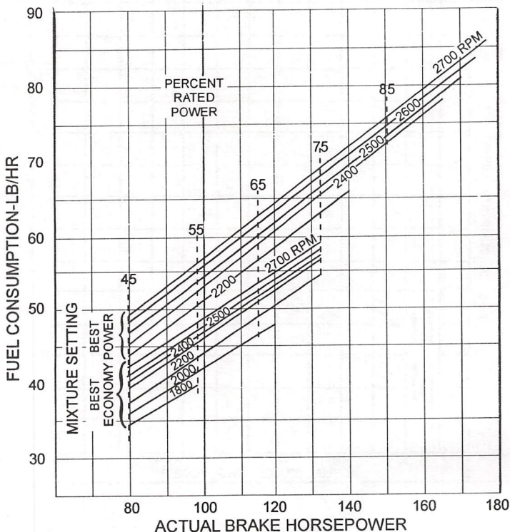
Figure 3-9. Part Throttle Fuel Consumption - IO-360-B1C
