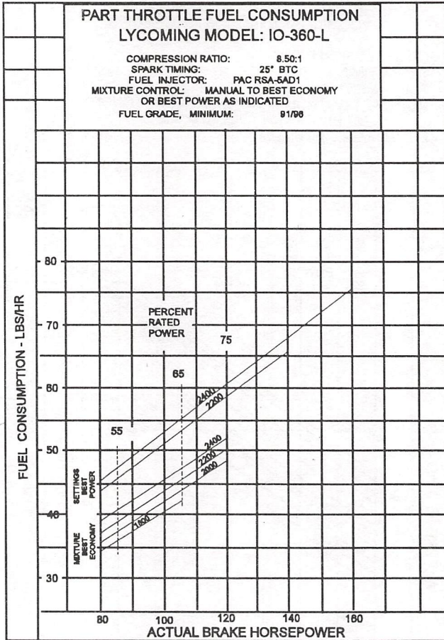
Figure 3-9A. Part Throttle Fuel Consumption - IO-360-L2A
