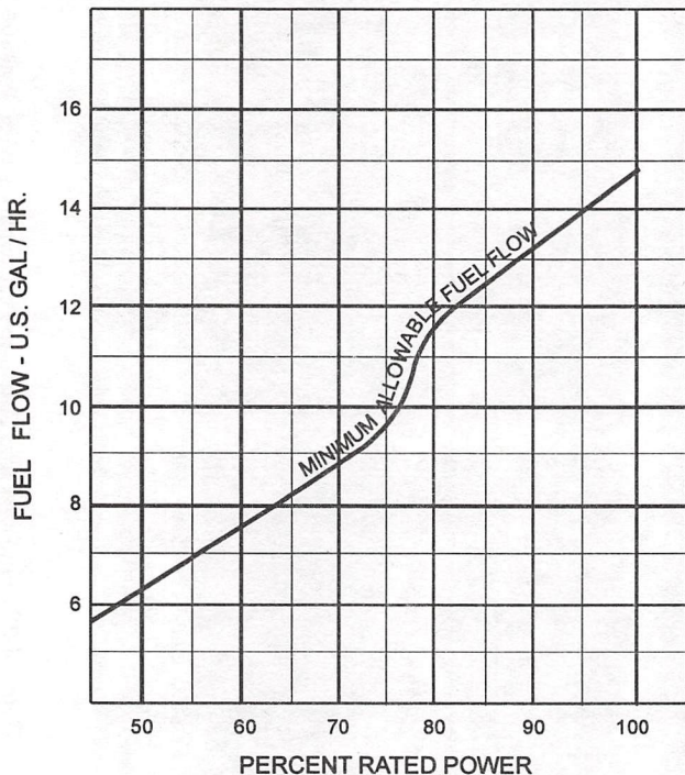
Figure 3-34. Fuel Flow vs Percent Rated Power O-360-A, -C, -F, -G Series; HO-360-C1A
