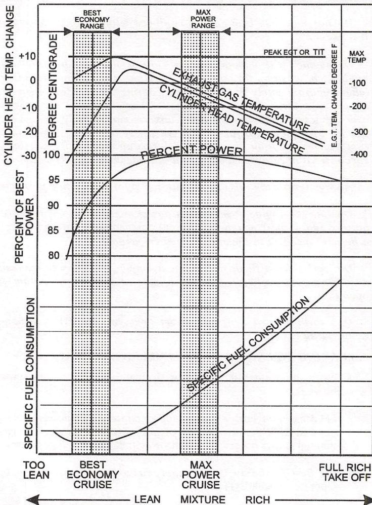
Figure 3-1. Representative Effect of Fuel/Air Ratio on Cylinder Head Temperature, Power and Specific Fuel Consumption at Constant RPM and Manifold Pressure in Cruise Range Operation
