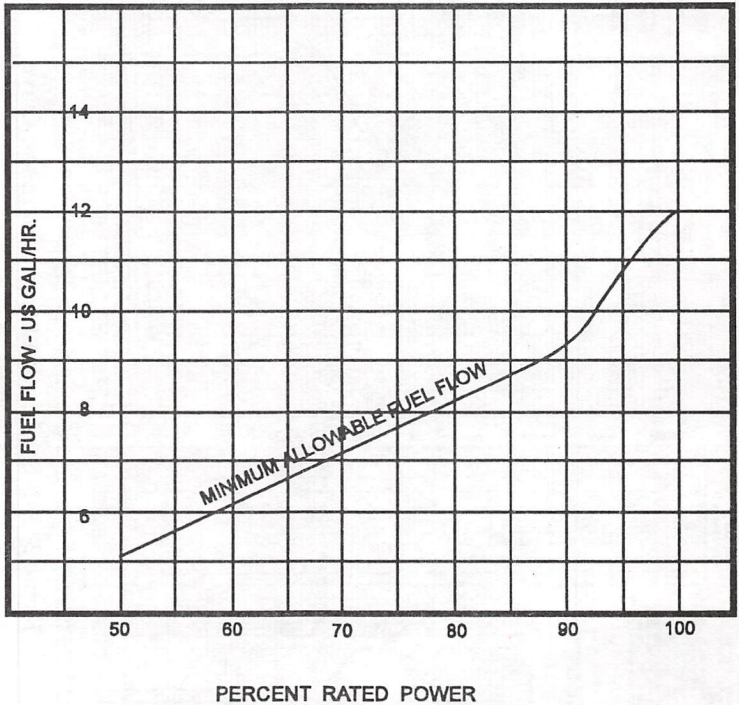
Figure 3-34A. Fuel Flow vs Percent Rated Power- O-360-J2A
