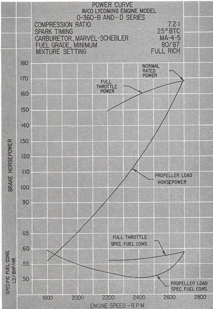
Figure 3-3. Power Curve - O-360-B, -D Series
