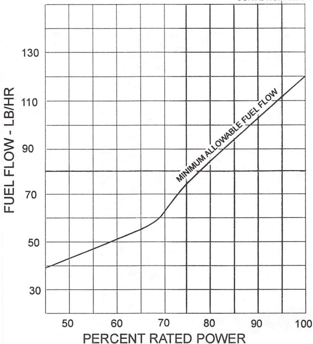
Figure 3-10. Fuel Flow vs Percent Rated Power - TIO-360-A Series
