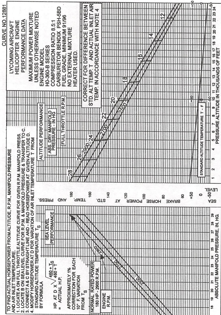
Figure 3-20. Sea Level and Altitude Performance - HO-360-B Series
