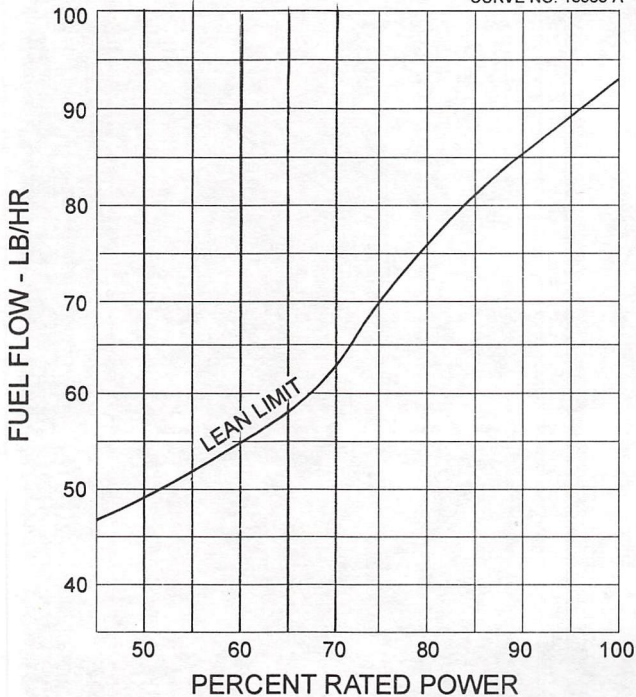
Figure 3-11. Fuel Flow vs Percent Rated Power - HIO-360-D Series
